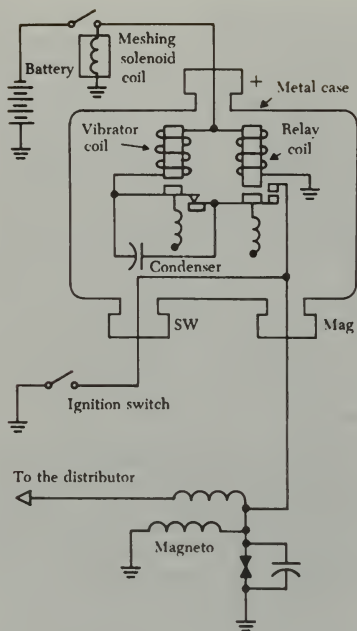
FIGURE 4-22. Induction vibrator.
